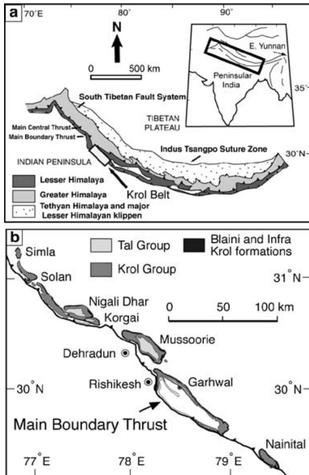
Figure 1. (a) Location of the Krol Belt within the Indian subcontinent and the Himalayan region. (b) Distribution of the various synclines within the Krol Belt that contain the Tal Group (modified from Jiang et al. 2002, fig. 2).
