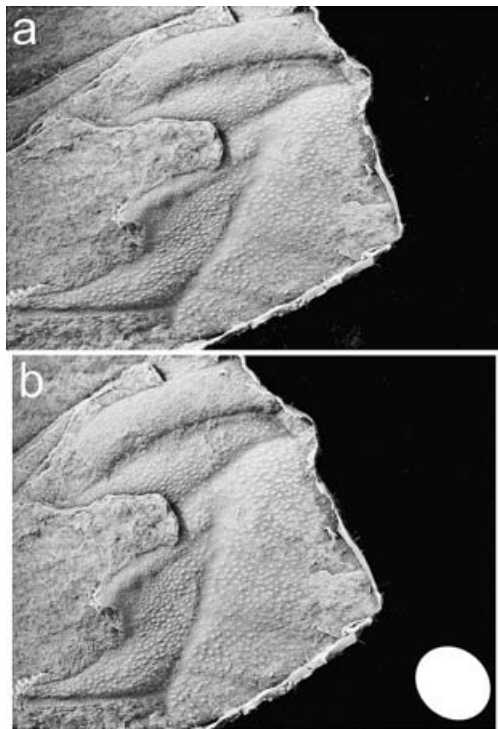
Figure 6. Original (a) and retrodeformation (b) of a latex mould of the external surface of the holotype cranium of Drepanopyge gopeni sp. nov. GSI 21150b, \times 1 . Ellipse represents the inverse of the strain ellipse (see Hughes, 1999 for procedural details).
