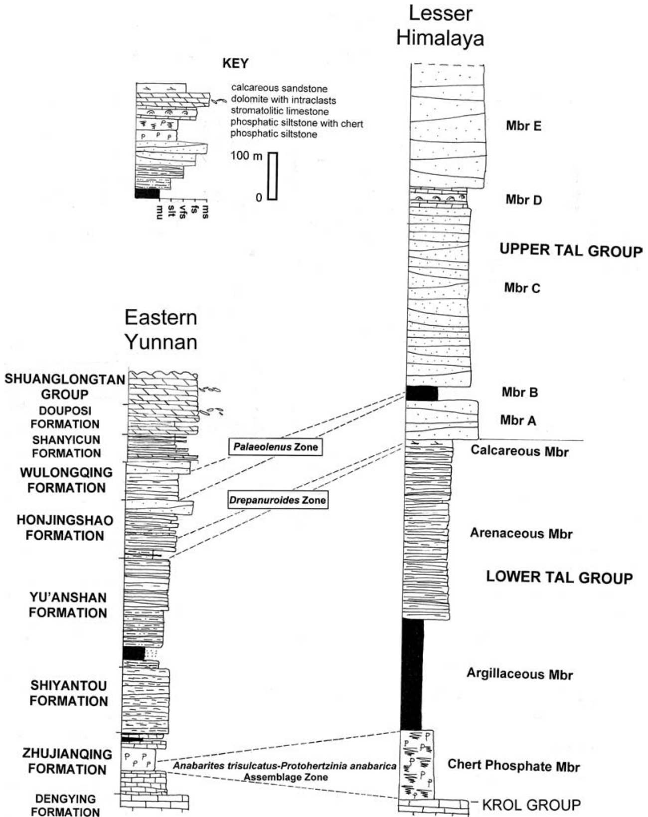
Figure 4. A generalized comparison of Cambrian successions from the Kunming region of southwest China and the Tal Group. The Chinese section was constructed from estimates of formation thickness in Luo (1974), Zhang (1988) and Zhu et al. (2001), and it should be noted that, as in the Tal Group, unit thickness varies between sections. Zones are correlated on the basis of diagnostic fossils discussed in the text. In the key the lowest five beds are siliciclastic: mu – mudstone, slt – siltstone, vfs – very fine grain sandstone, fs – fine grain sandstone, ms – medium grain sandstone.
