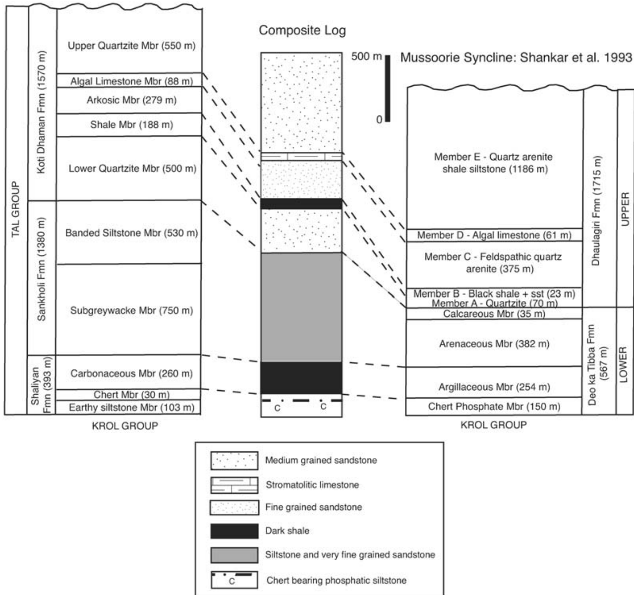
Figure 2. Lithostratigraphy of the Tal Group, showing recent schemes for the Nigali Dhar syncline in the northwestern region (Bhargava et al. 1998), and the Mussoorie syncline in the southeast region (Shanker et al. 1993). Although thickness estimates and stratigraphic hierarchies differ in the two regions, a broadly similar succession of lithotypes can be recognized throughout the region. Poor exposure and structural complexity hinders characterization of these units and thickness estimates can vary widely (Shanker, Kumar & Saxena, 1989, table 6A).
