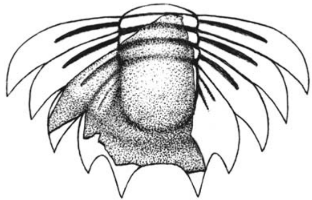
Figure 7. Comparison of the fragmentary pygidium of Drepanopyge gopeni sp. nov. GSI 20698 (Fig. 5d) with that of Drepanopyge mirabilis Lu, showing the close similarity of preserved portions of the Indian material with the Chinese species.
