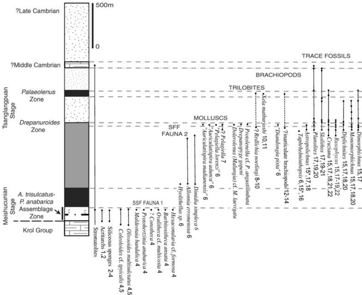
Figure 3. Summary of the distribution of fossils within the Tal Group. The choice of taxa and taxonomic level represented reflects the authors' opinions as to the potential biostratigraphic utility of forms described. Inverted commas around taxonomic names imply that taxonomic attribution at this level is questionable. * Implies that the record is questionably assigned to that ichnotype. The stratigraphic placement of fossils within the upper parts of the Sankholi Formation or Deo ka Tibba Formation (Fig. 2) is uncertain in some cases (see text). Given thickness and lithostratigraphic differences within the outcrop belt positioning is somewhat approximate. Sources: 1 – Prasad et al. 1990; 2 – Tiwari, 1999; 3 – Mazumdar & Banerjee, 1998; 4 – Brasier & Singh, 1987; 5 – Bhatt & Mathur, 1990b; 6 – Kumar et al. 1983; 7 – Mathur & Srivastava, 1994; 8 – Kumar, Joshi & Mathur, 1987; 9 – Joshi, Mathur & Bhatt, 1989; 10 – Jell & Hughes, 1997; 11 – Mathur & Joshi, 1989b; 12 – Tripathi et al. 1984; 13 – Tripathi et al. 1986; 14 – Mathur & Joshi, 1989a; 15 – Singh & Rai, 1983; 16 – Banerjee & Narain, 1976; 17 – Bhargava et al. 1998; 18 – Mathur, Joshi & Kumar, 1988; 19 – Rai, 1987; 20 – De, Das & Raha, 1994; 21 – Bhargava, 1984; 22 – Joshi & Mathur, 1987. Ornament in stratigraphic column as for Figure 2.
