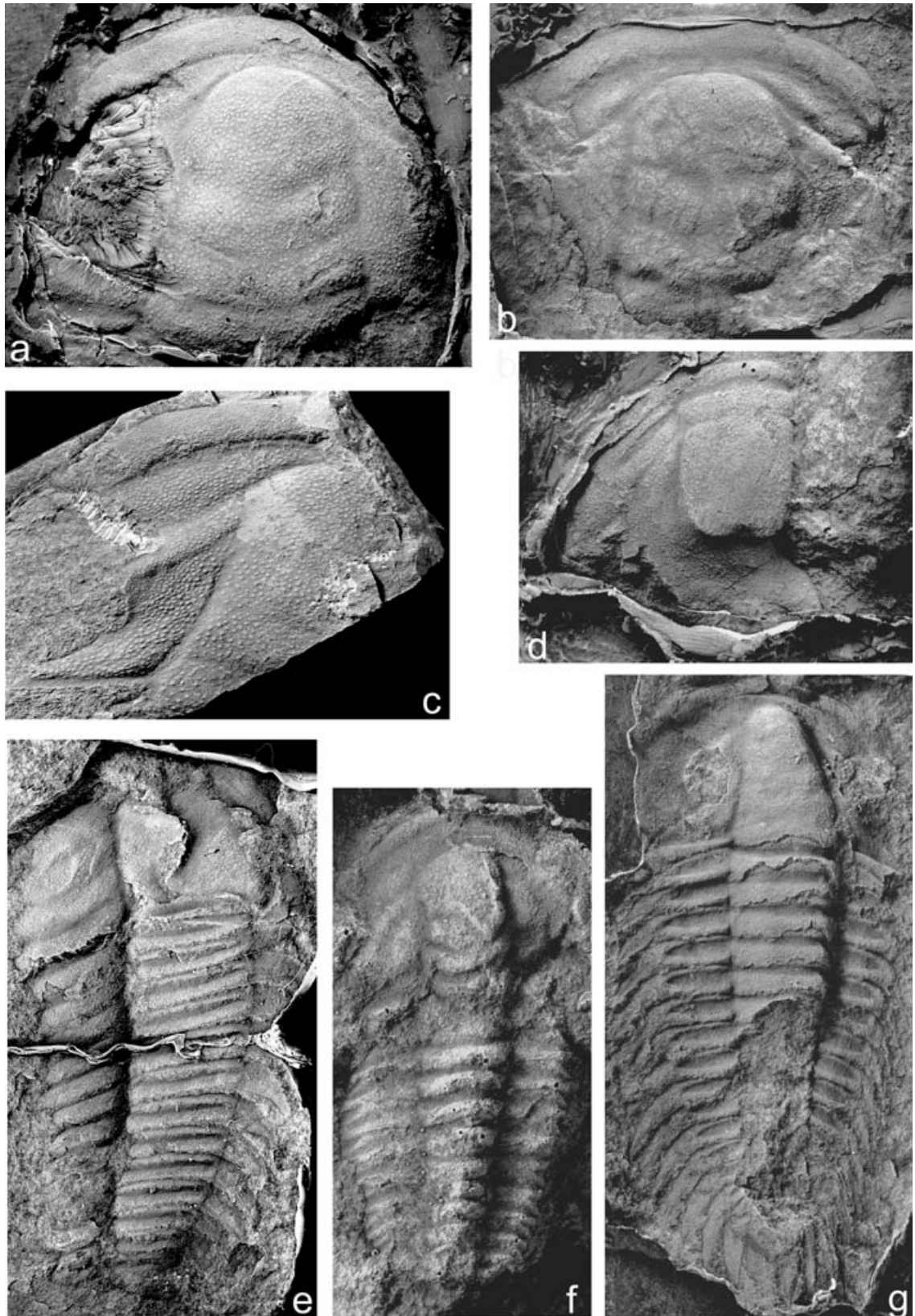
Figure 5. Trilobites from collection P2, uppermost Sankholi Formation in Pirtari–Dochi Section, Sirmaur district, Himachal Pradesh, India. All specimens coated with ammonium chloride sublimate prior to photography, specimens are internal surfaces of composite moulds unless otherwise stated. (a–e) Drepanopyge gopeni sp. nov., (a) GSI 20696 (CMCP50115), partial cranidium, \times 1.5 , (b) GSI 20697 (CMCP50116), partial cranidium, \times 1.5 , (c) GSI 21150a (CMCP50120), partial cranidium, original specimen, holotype, \times 1.5 , (d) GSI 20698 (CMCP50117), partial pygidium, \times 2 , (e) GSI 21151 (CMCP50121), partial cephalon and anterior trunk, latex cast of external surface of composite mould, \times 2 , (f) Protolenella cf. P. angustilimbata Qian & Yao, GSI 20699 (CMCP50118), cranidium and anterior trunk, \times 6 , (g) Dolerolenus ( Malungia ) cf. M. laevigata Lu, counterpart of dorsal exoskeleton, GSI 20700 (CMCP50119), \times 2.5 .
